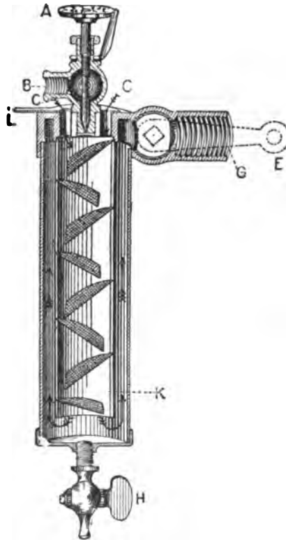
FIG. 320.- The "Auto" Carburettor. A , wheel controlling needle valve; B , gasoline inlet; C , C , air inlets; E , throttle lever; G , pipe to cylinder; H , drip cock; K , inner cylinder containing segments of wire gauze; L , valve controlling air inlets.
